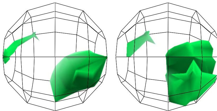
(a) Nucleation
